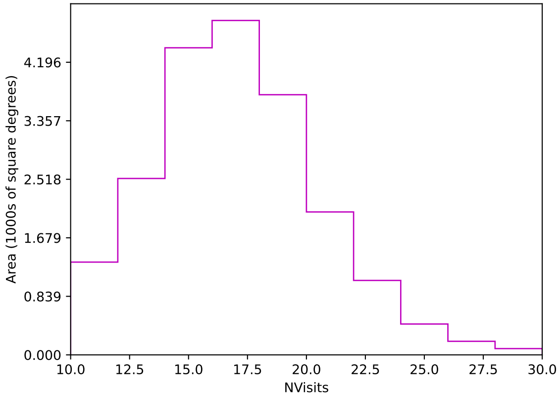
extra_ss_neo4_v3.4_10yrs Yr 1 z band: NVisits
