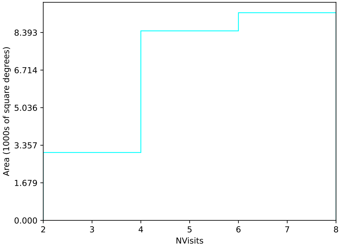
extra_ss_neo4_v3.4_10yrs Yr 1 u band: NVisits
