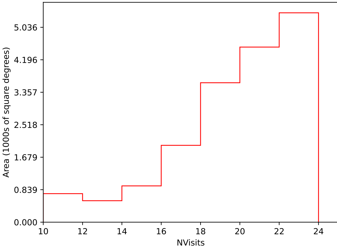
extra_ss_neo4_v3.4_10yrs Yr 1 i band: NVisits
