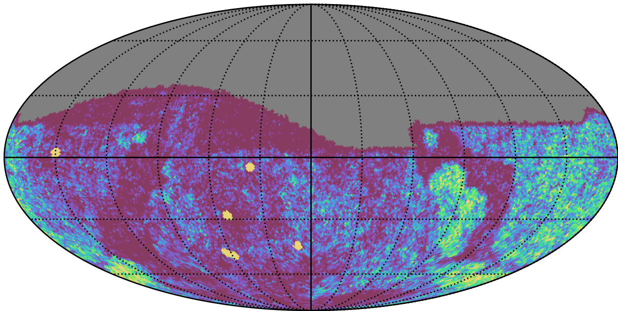
extra_ss_neo4_v3.4_10yrs Yr 1 g band: NVisits
