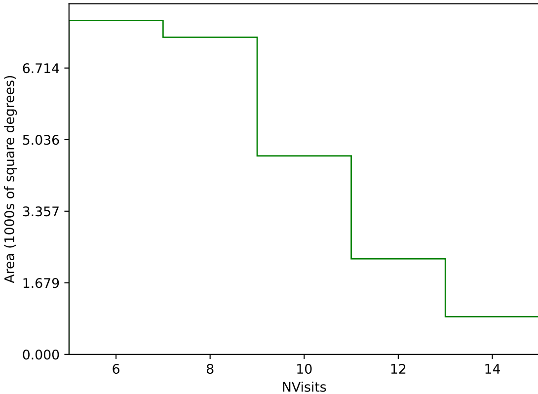
extra_ss_neo4_v3.4_10yrs Yr 1 g band: NVisits
