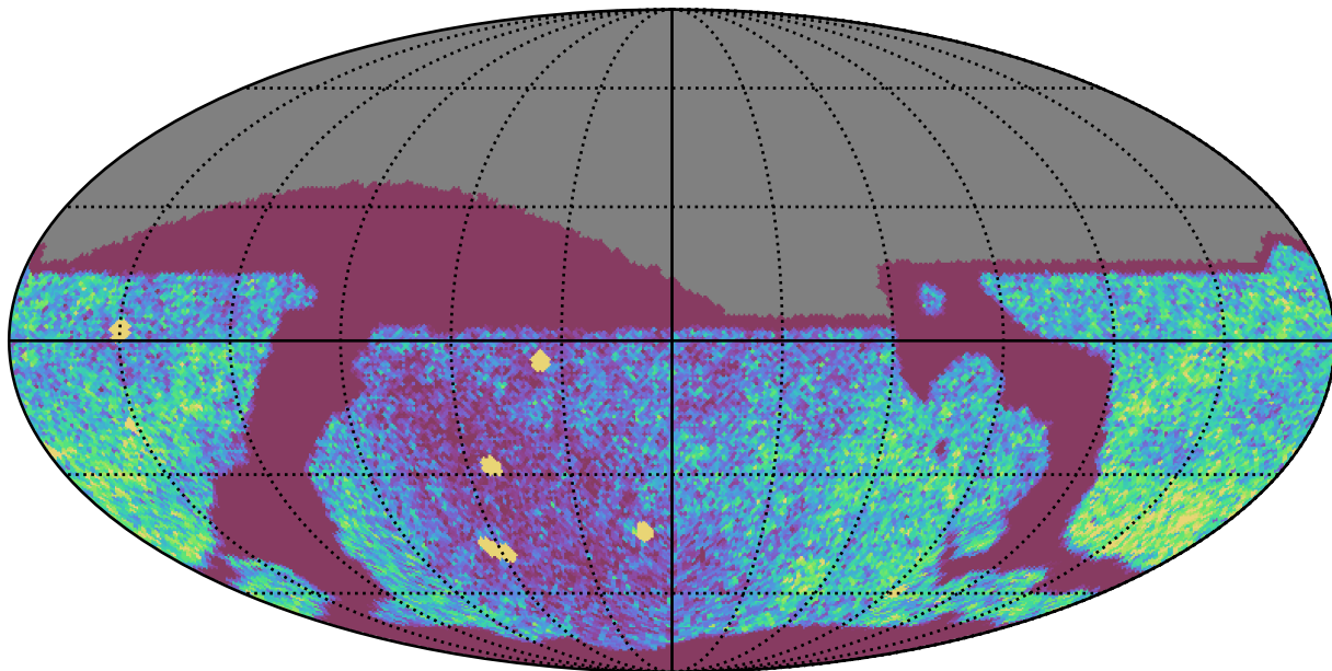
extra_ss_neo4_v3.4_10yrs Yr 1 all bands: NVisits
