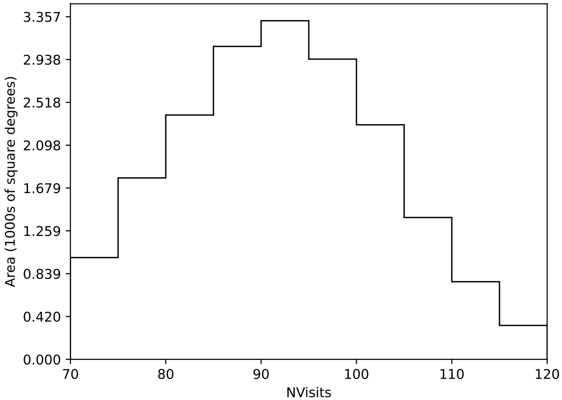
extra_ss_neo4_v3.4_10yrs Yr 1 all bands: NVisits
