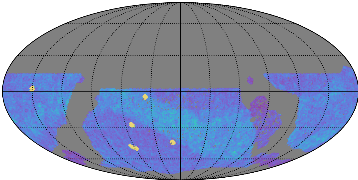
extra_ss_neo4_v3.4_10yrs WFD z band: NVisits
