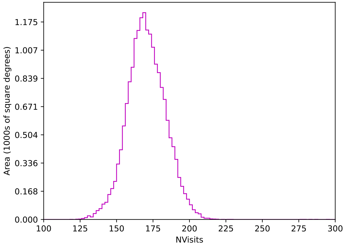
extra_ss_neo4_v3.4_10yrs WFD z band: NVisits
