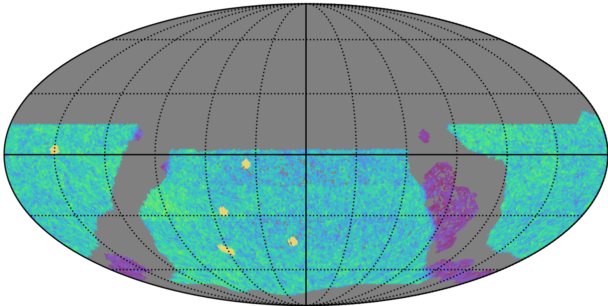
extra_ss_neo4_v3.4_10yrs WFD u band: NVisits
