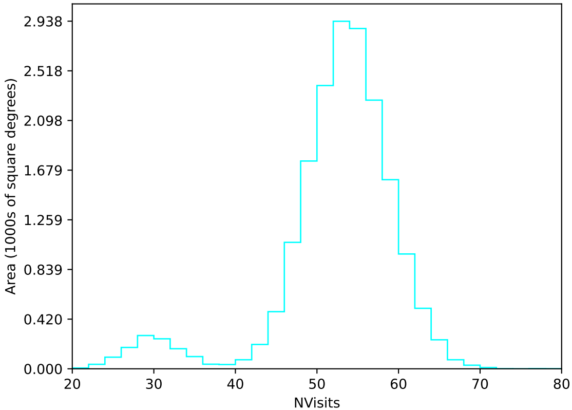
extra_ss_neo4_v3.4_10yrs WFD u band: NVisits
