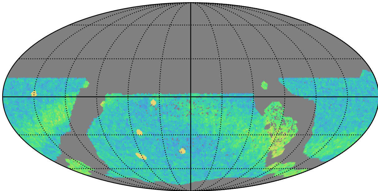
extra_ss_neo4_v3.4_10yrs WFD r band: NVisits
