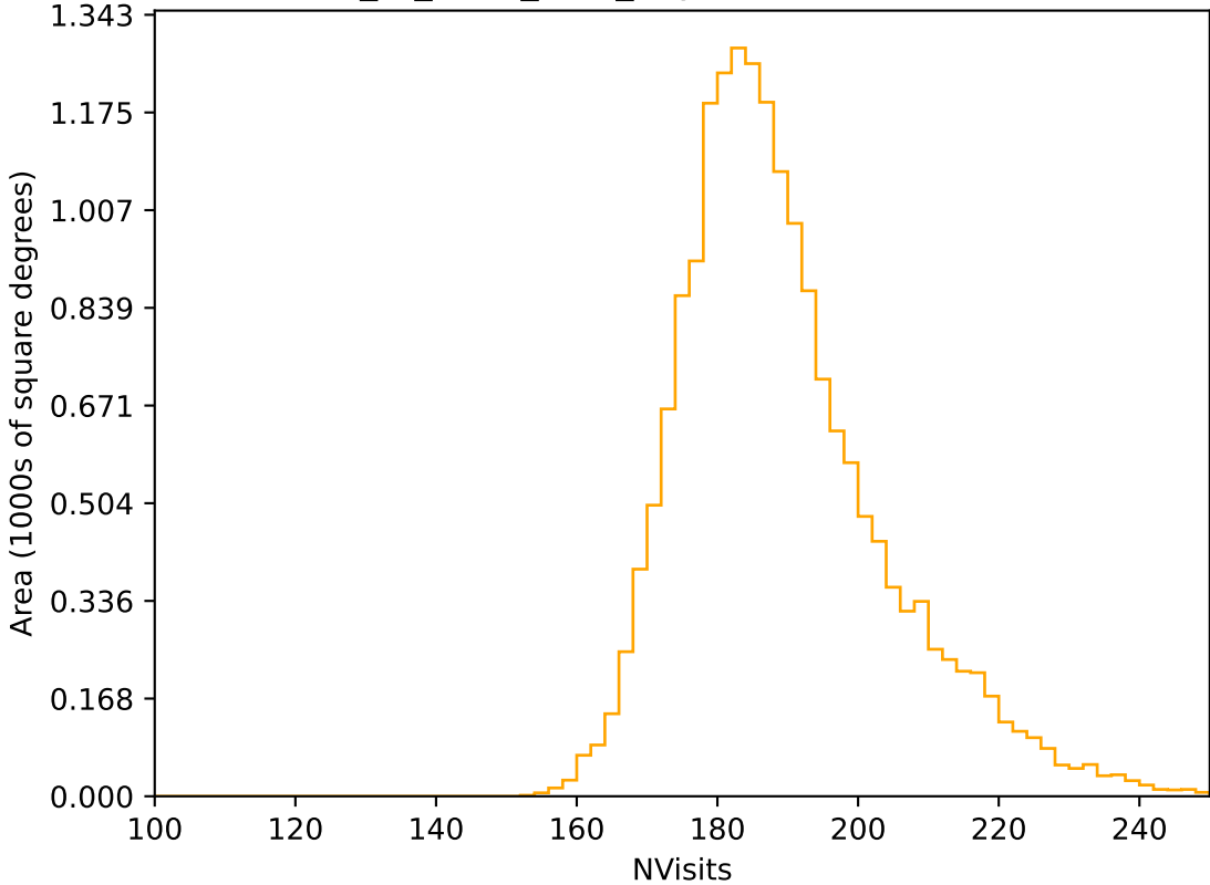
extra_ss_neo4_v3.4_10yrs WFD r band: NVisits
