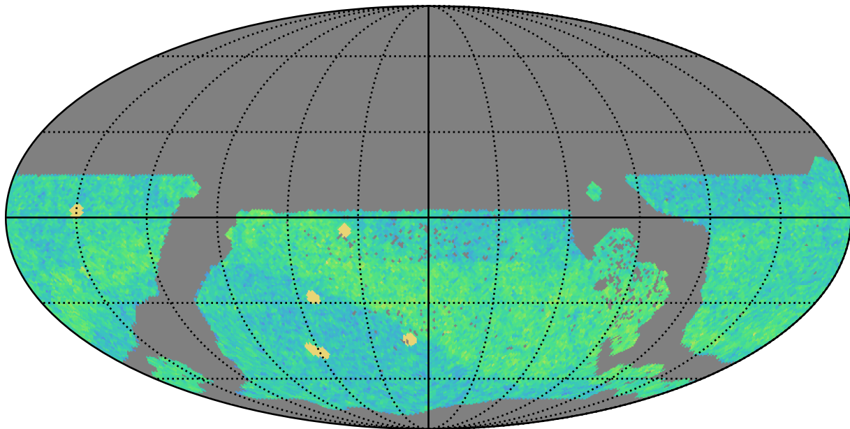
extra_ss_neo4_v3.4_10yrs WFD i band: NVisits
