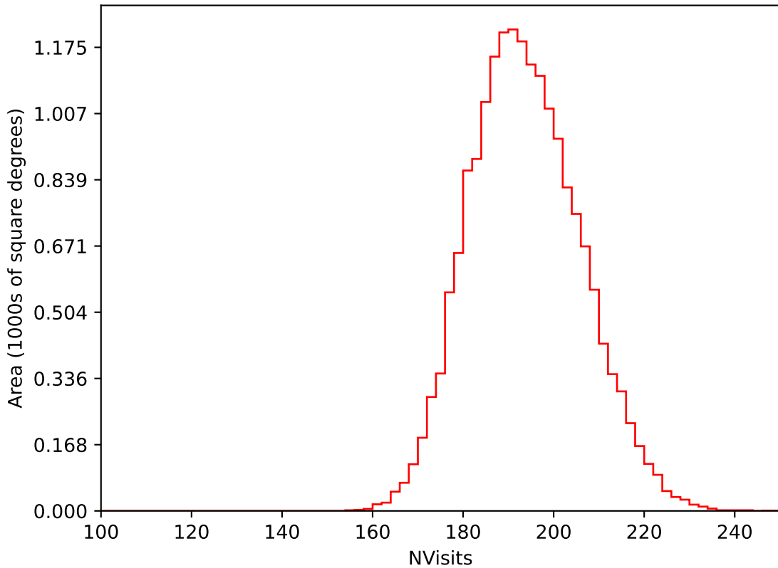
extra_ss_neo4_v3.4_10yrs WFD i band: NVisits
