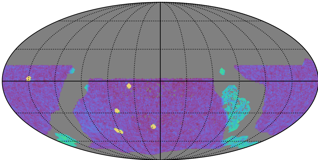
extra_ss_neo4_v3.4_10yrs WFD g band: NVisits
