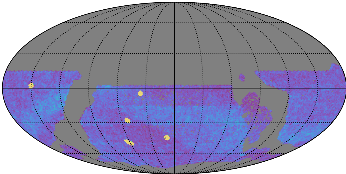
extra_ss_neo4_v3.4_10yrs WFD all bands: NVisits
