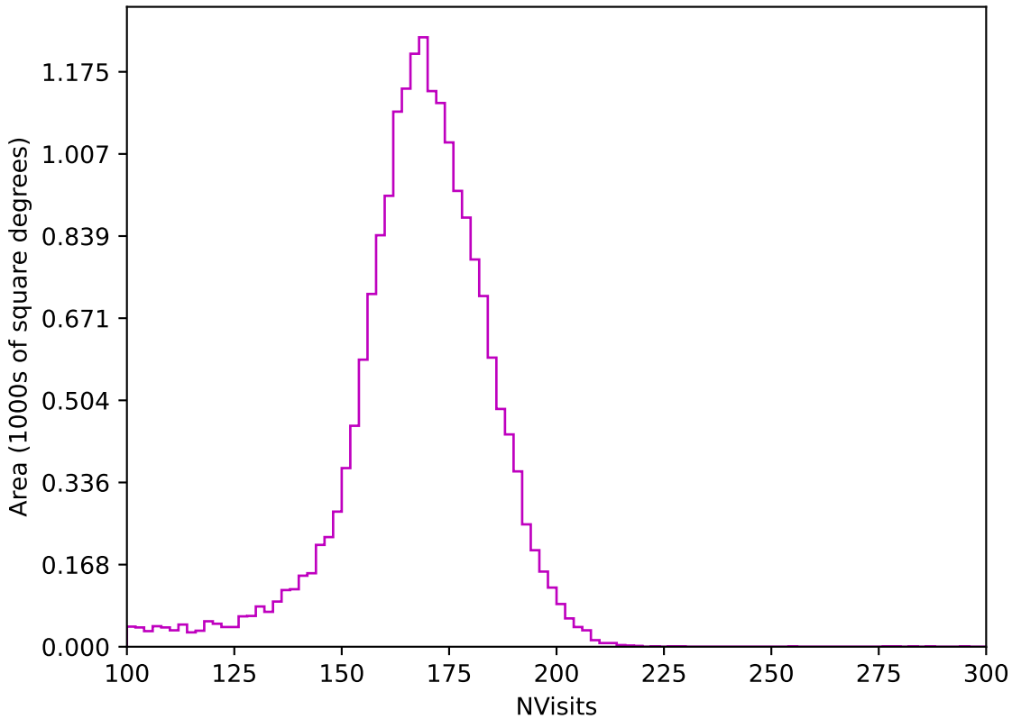
extra_ss_neo4_v3.4_10yrs All sky z band: NVisits
