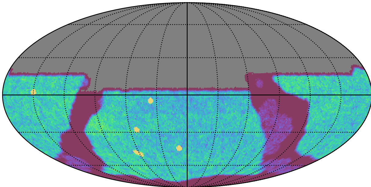
extra_ss_neo4_v3.4_10yrs All sky u band: NVisits
