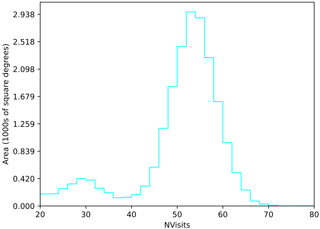
extra_ss_neo4_v3.4_10yrs All sky u band: NVisits
