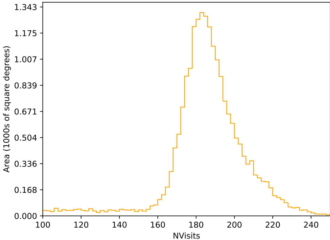
extra_ss_neo4_v3.4_10yrs All sky r band: NVisits
