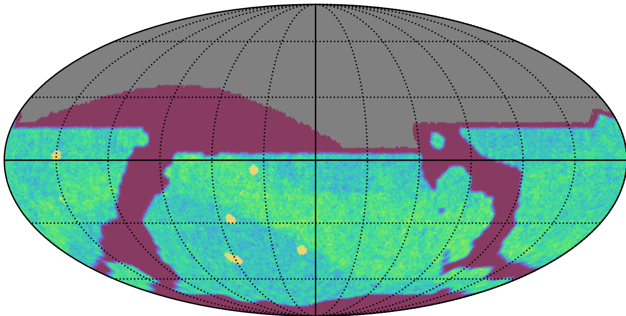
extra_ss_neo4_v3.4_10yrs All sky i band: NVisits
