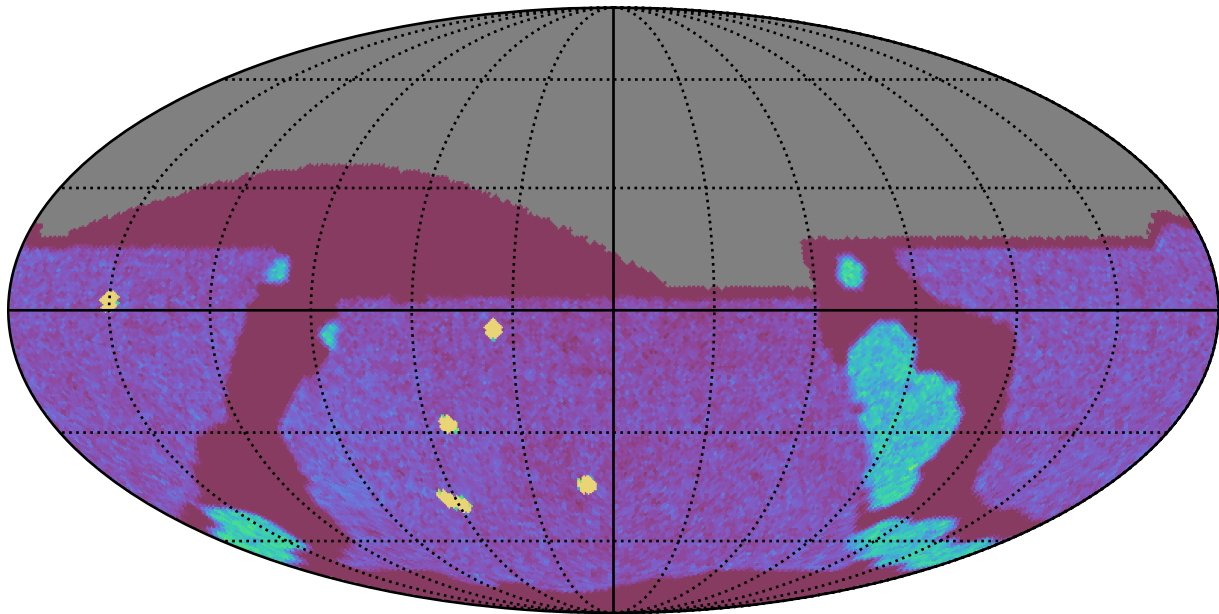
extra_ss_neo4_v3.4_10yrs All sky g band: NVisits
