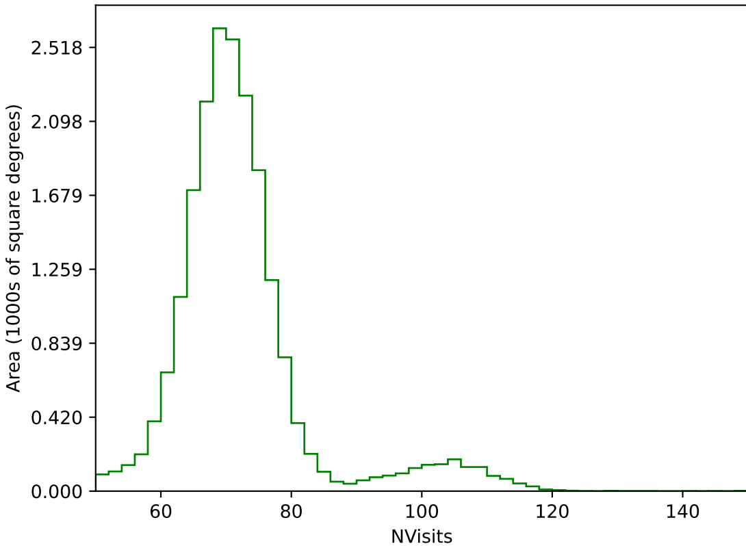
extra_ss_neo4_v3.4_10yrs All sky g band: NVisits
