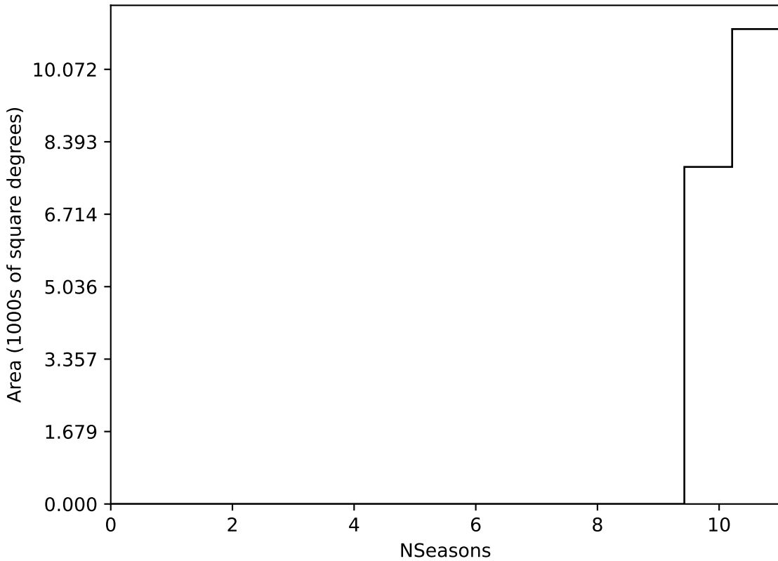
extra_ss_neo4_v3.4_10yrs WFD all bands: NSeasons
