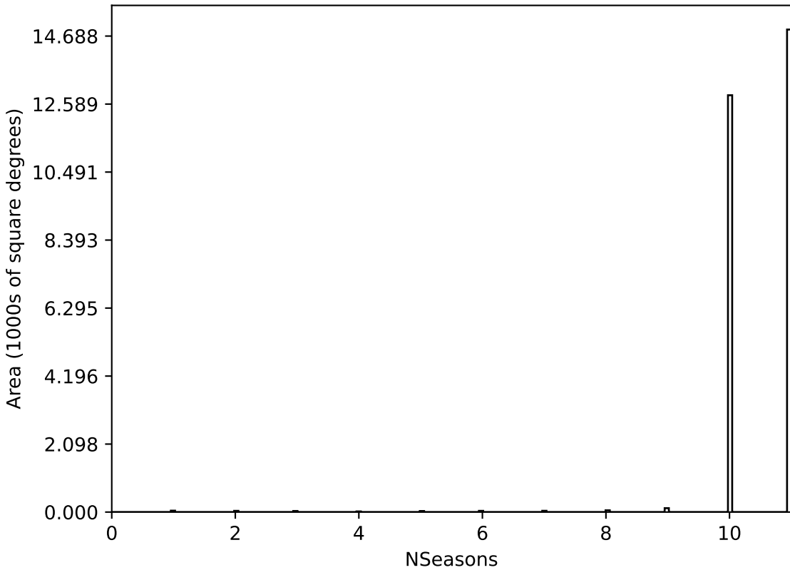
extra_ss_neo4_v3.4_10yrs All sky all bands: NSeasons
