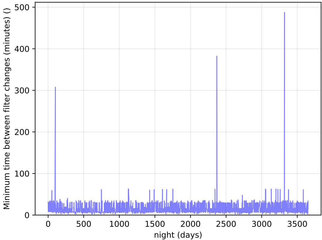
extra_ss_neo4_v3.4_10yrs Per Night: Minimum time between filter changes (minutes)
