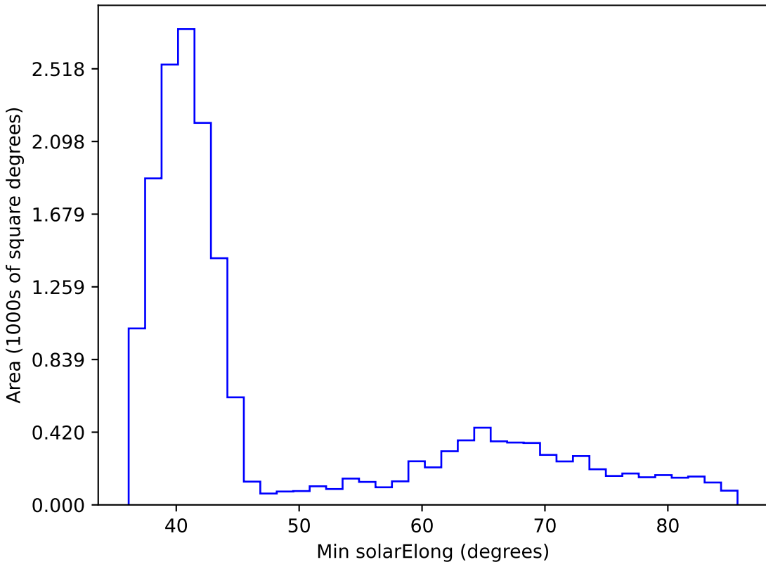
extra_ss_neo4_v3.4_10yrs WFD z band: Min solarElong
