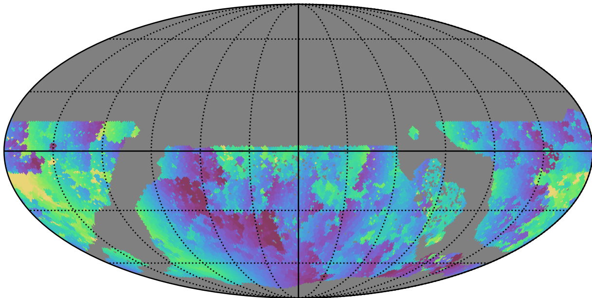
extra_ss_neo4_v3.4_10yrs WFD u band: Min solarElong
