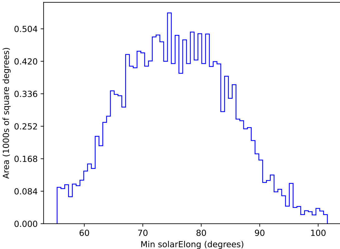
extra_ss_neo4_v3.4_10yrs WFD u band: Min solarElong
