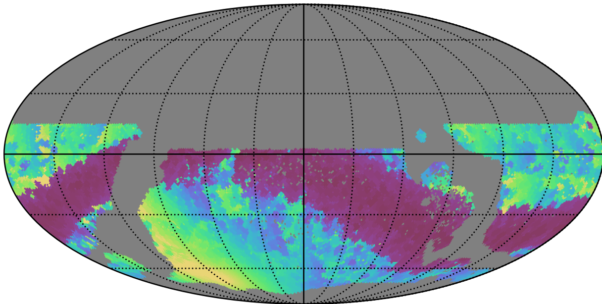
extra_ss_neo4_v3.4_10yrs WFD r band: Min solarElong
