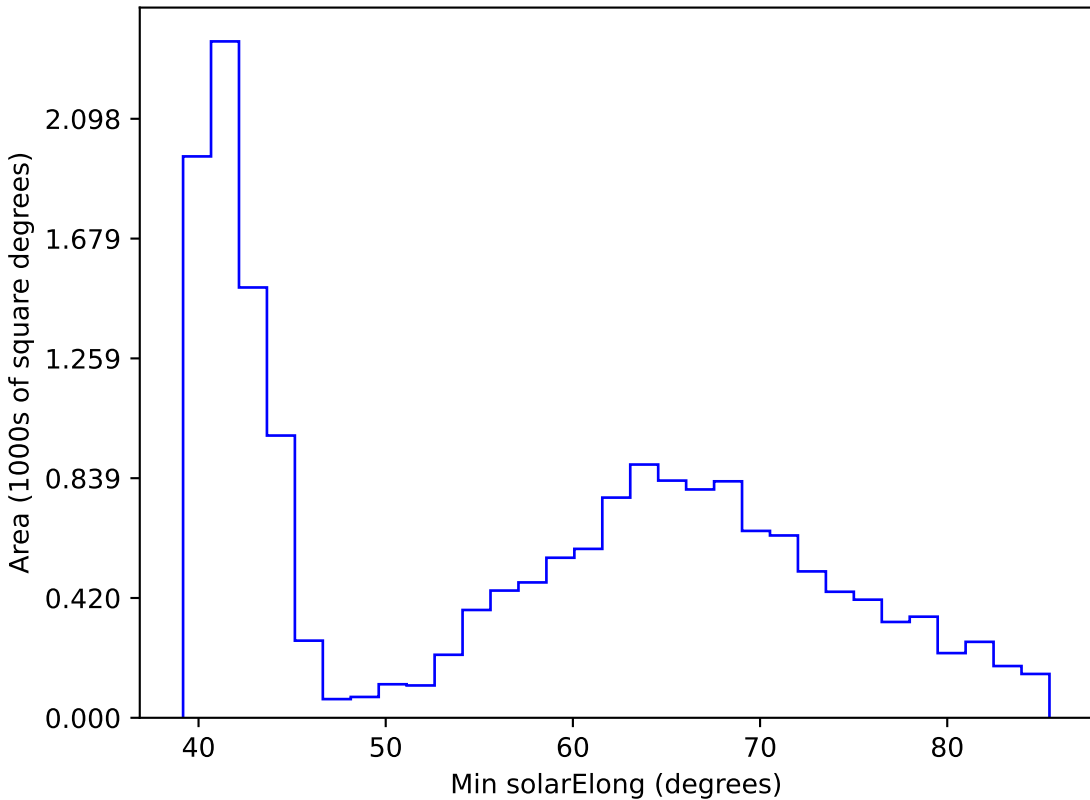
extra_ss_neo4_v3.4_10yrs WFD r band: Min solarElong
