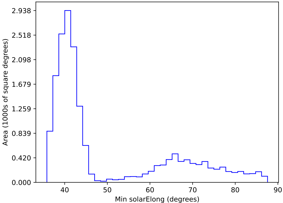
extra_ss_neo4_v3.4_10yrs WFD i band: Min solarElong
