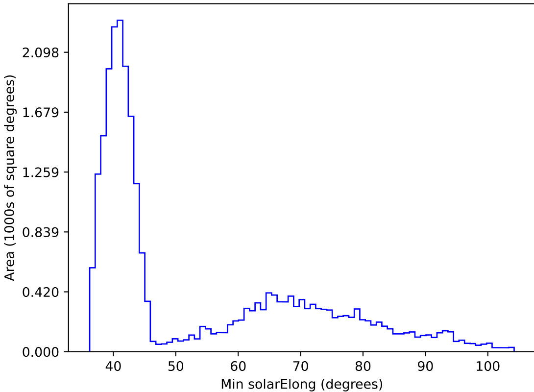
extra_ss_neo4_v3.4_10yrs All sky z band: Min solarElong
