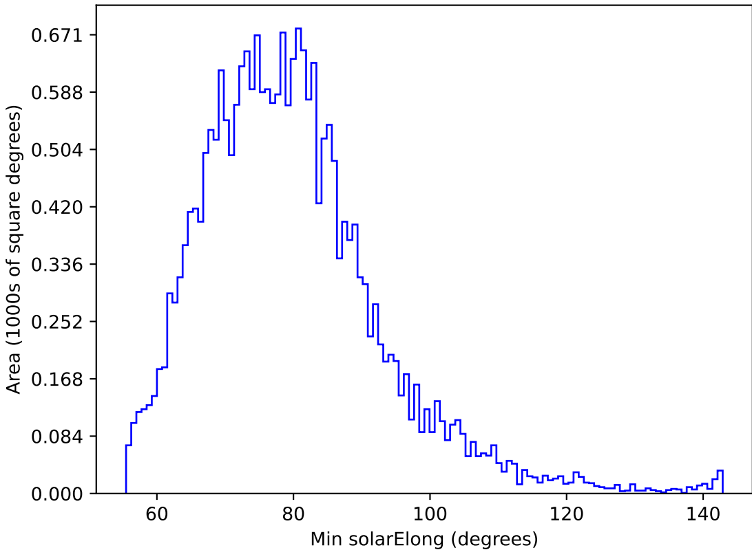
extra_ss_neo4_v3.4_10yrs All sky u band: Min solarElong
