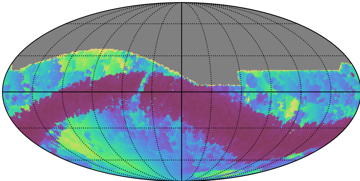
extra_ss_neo4_v3.4_10yrs All sky r band: Min solarElong
