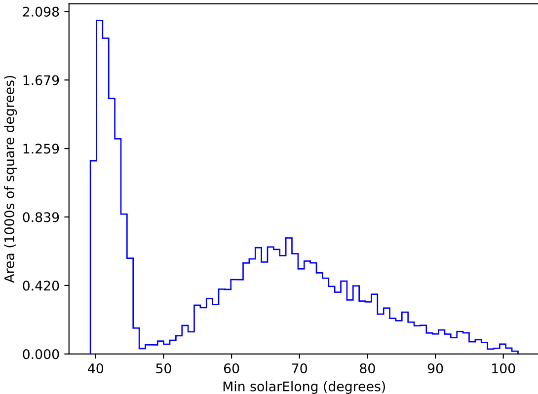
extra_ss_neo4_v3.4_10yrs All sky r band: Min solarElong
