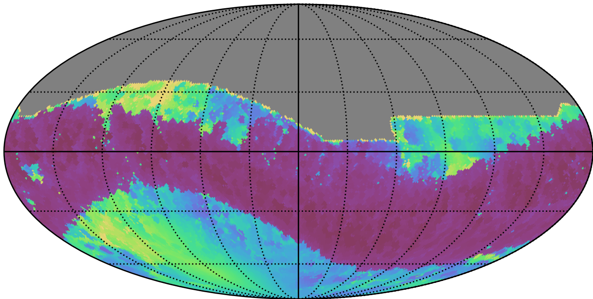
extra_ss_neo4_v3.4_10yrs All sky i band: Min solarElong
