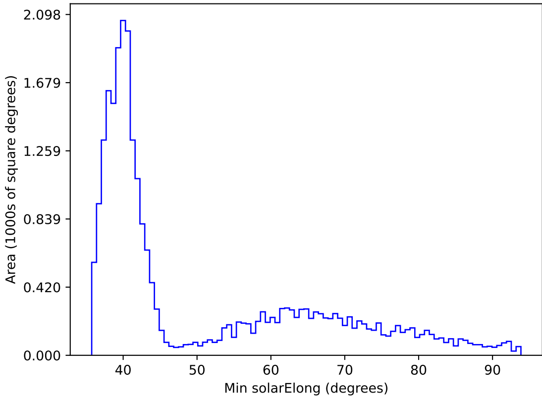
extra_ss_neo4_v3.4_10yrs All sky all bands: Min solarElong
