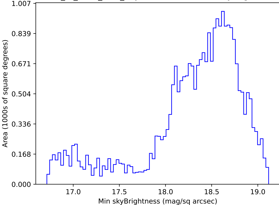
extra_ss_neo4_v3.4_10yrs Yr 1 z band: Min skyBrightness
