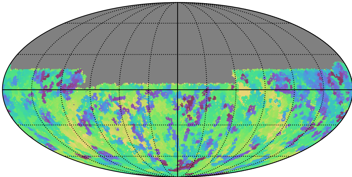
extra_ss_neo4_v3.4_10yrs Yr 1 y band: Min skyBrightness
