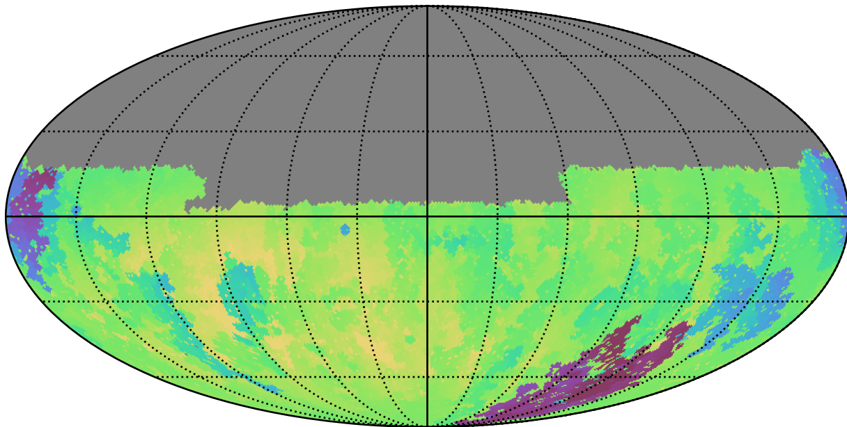
extra_ss_neo4_v3.4_10yrs Yr 1 u band: Min skyBrightness
