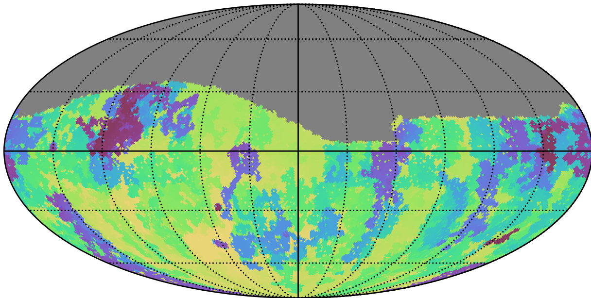
extra_ss_neo4_v3.4_10yrs Yr 1 g band: Min skyBrightness
