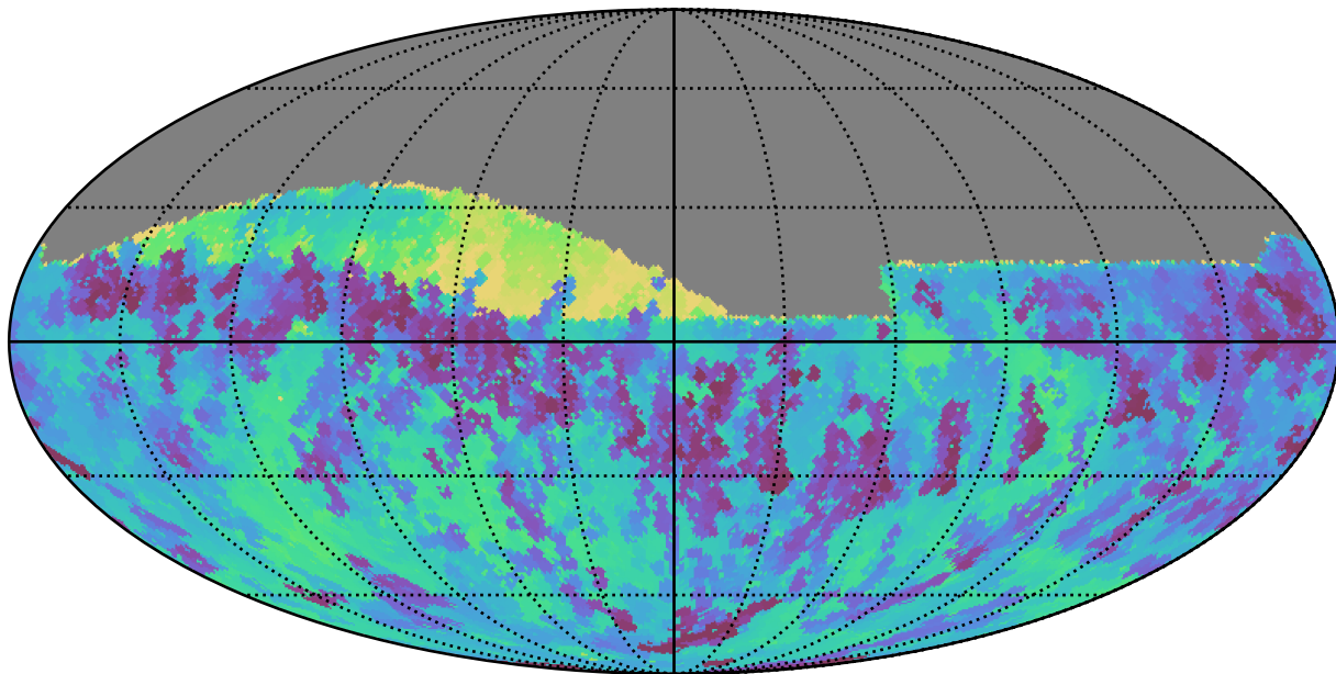
extra_ss_neo4_v3.4_10yrs Yr 1 all bands: Min skyBrightness
