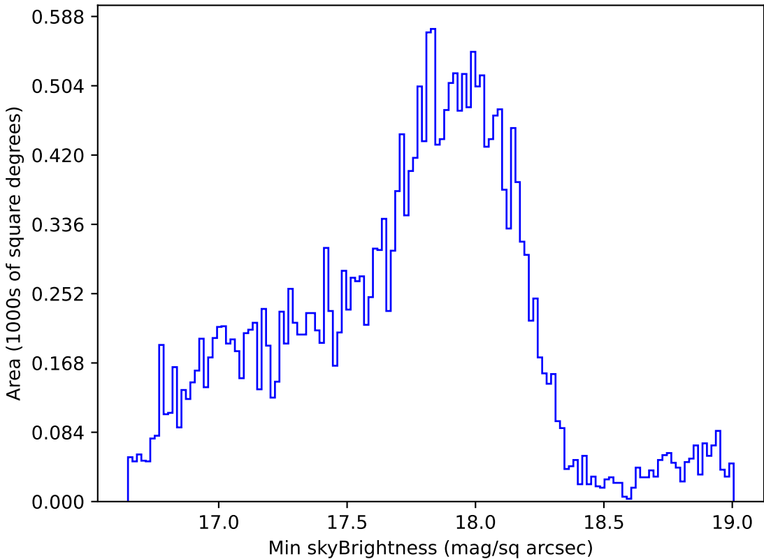
extra_ss_neo4_v3.4_10yrs Yr 1 all bands: Min skyBrightness
