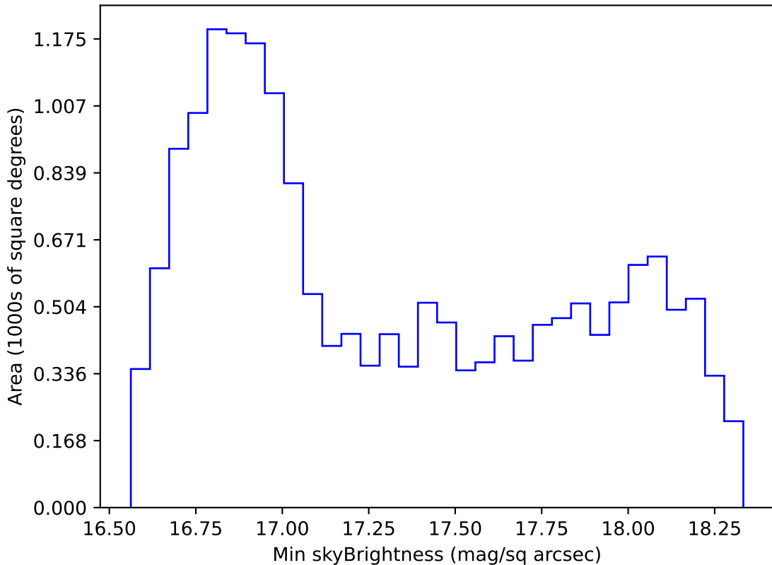
extra_ss_neo4_v3.4_10yrs WFD z band: Min skyBrightness
