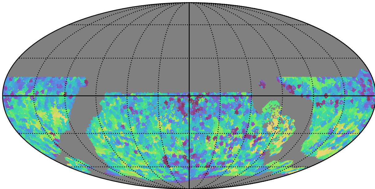
extra_ss_neo4_v3.4_10yrs WFD y band: Min skyBrightness
