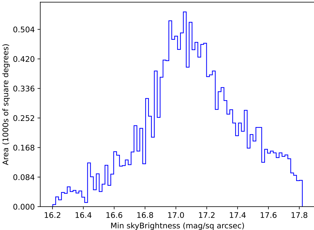
extra_ss_neo4_v3.4_10yrs WFD y band: Min skyBrightness
