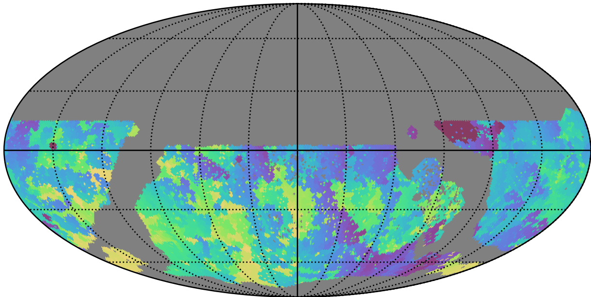
extra_ss_neo4_v3.4_10yrs WFD u band: Min skyBrightness
