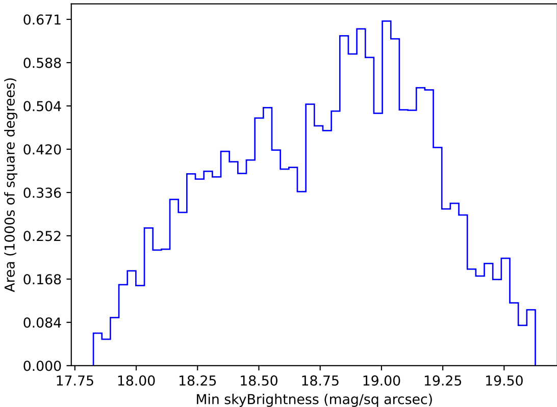
extra_ss_neo4_v3.4_10yrs WFD r band: Min skyBrightness
